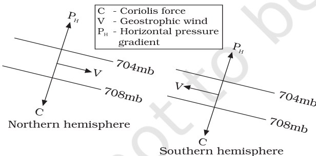
Figure 9.4 : Geostrophic Wind
